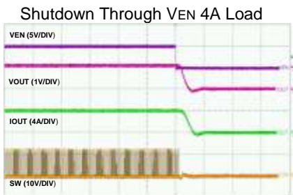
Time-50μs/div
